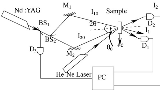
Fig. 3. Experimental setup of holographic storage. M 1 , M 2 : mirrors; BS 1 , BS 2 : beam splitters; D 1 –D 3 : detectors.
