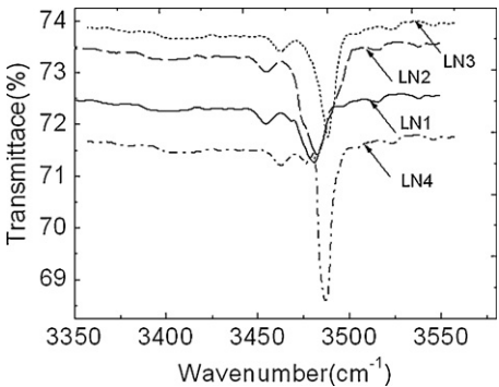
Fig. 4. The infrared absorption spectra of Hf:Fe:Mn:LiNbO 3 crystals.
