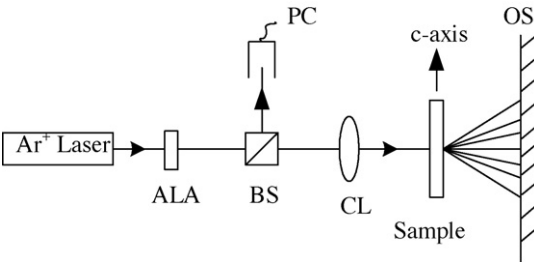
Fig. 2. Experimental setup of the light-scattering resistance ability. ALA: adjustable light attenuator, BS: beam splitter, PC: photodiode, CL: convex lens, OS: observation screen.
